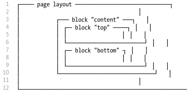
Listing 12-3
