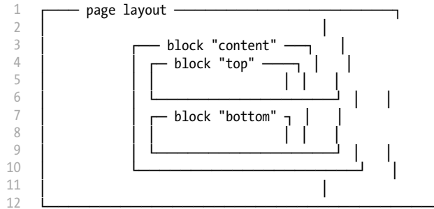
Listing 12-3
