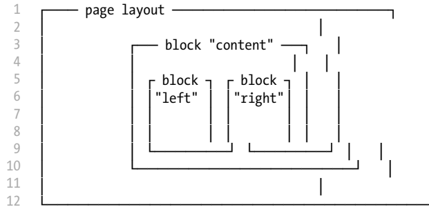
Listing 12-4
