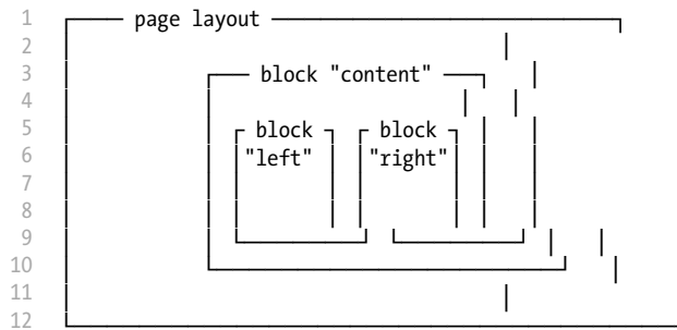
Listing 12-4
